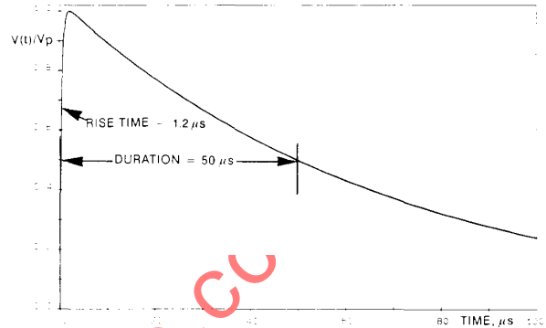
Fig 12 Combination Wave, Open-Circuit Voltage
