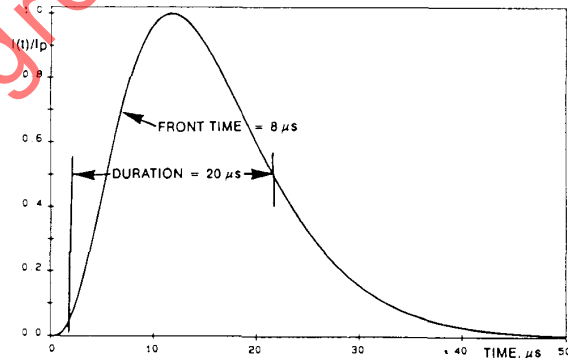
Fig 13 Combination Wave, Short-Circuit Current
